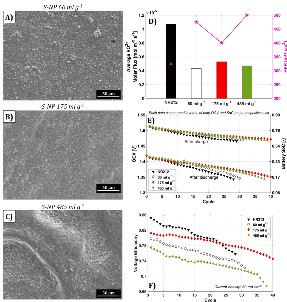
Fig. 3. SEM images of barrier layers top-view on silicon wafers at different S-NP: A) 60 \text{ml g}^{-1} , B) 175 \text{ml g}^{-1} and C) 485 \text{ml g}^{-1} . D) Average vanadium fluxes during diffusion test (left axis) and HFR (magenta markers, right axis) with barriers on Nafion™ NR212 at different S-NP and for the reference Nafion™ NR212. E) Battery OCV (left axis) and SoC (right axis) and F) Voltage Efficiency during charge-discharge cycles at fixed capacity with barriers at different S-NP and the reference Nafion™ NR212. (For interpretation of the references to colour in this figure legend, the reader is referred to the Web version of this article.)
