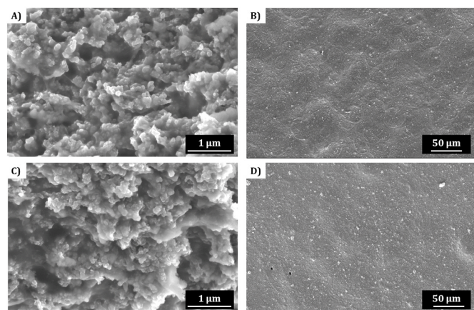
Fig. 4. – SEM images of barrier layers deposited on silicon wafers with different ink flow rate: A, B) 0.2 \text{ml min}^{-1} , cross-section view and top view respectively, and C, D) 0.5 \text{ml min}^{-1} , cross-section view and top view respectively.
