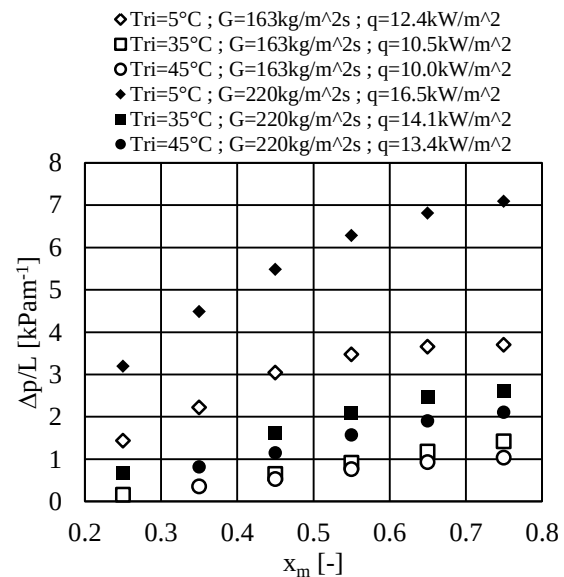
Figure 5. Pressure drop per unit length versus mean quality (quality change \Delta x=0.2 ).
