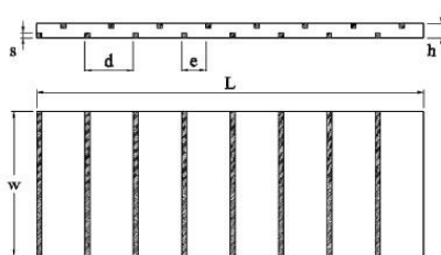
Figure 1. Ribbed channel geometry.
