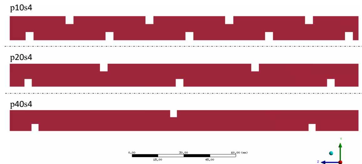
Figure 2. Channel configurations considered.
