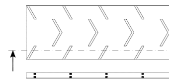
Figure 2(b). 3D_{up} and 3D_{down} : broken V-shaped ribs in upstream or downstream configuration.
