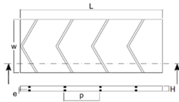
Figure 2(a). V_{up} : V-shaped ribs in upstream configuration.
