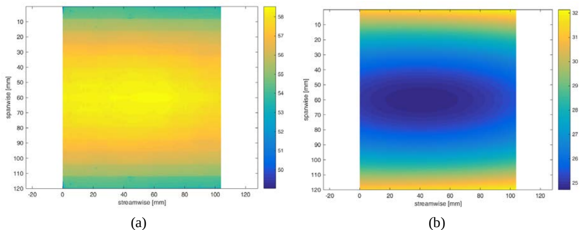
Figure 7. Temperature (a) and h (b) distribution for Re = 5400 , flat reference surface
