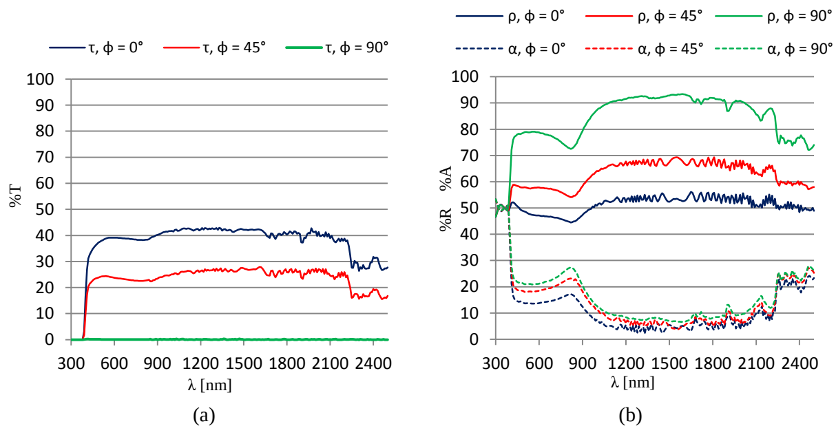
Figure 13. Transmittance (a), reflectance and absorptivity (b) vs. wavelength for a double WG film, various \varphi
