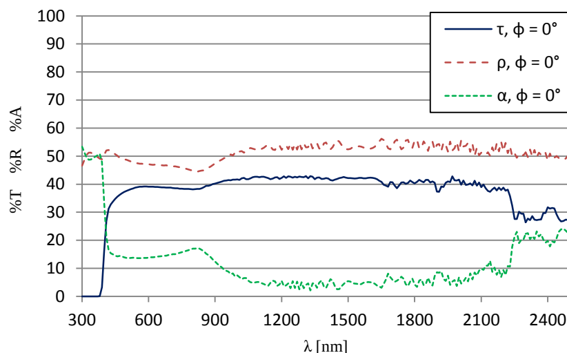
Figure 12. Transmittance, reflectance and absorptivity vs. wavelength for a double WG film, \varphi = 0^\circ
