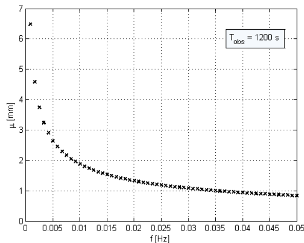
Figure 1. Thermal diffusion length, Plexiglas, fixed observation time
