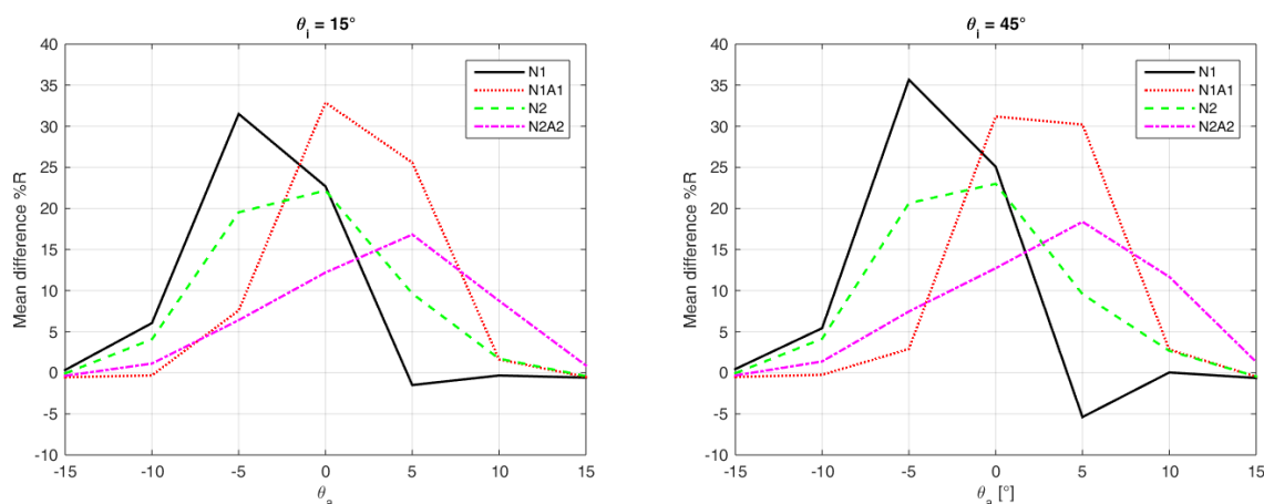
Figure 10. Average reflectance increase, Vis range, for \theta_i = 15^\circ and \theta_i = 45^\circ , at seven aspecular angles.
