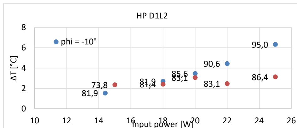
Figure 6. Temperature difference for HP D1L2 at various powers, for quasi-horizontal orientation, \phi = 0^\circ and \phi = -10^\circ ( \Delta z = 2.26 cm). Numbers near the points are the average temperature of the HP during the trial.
